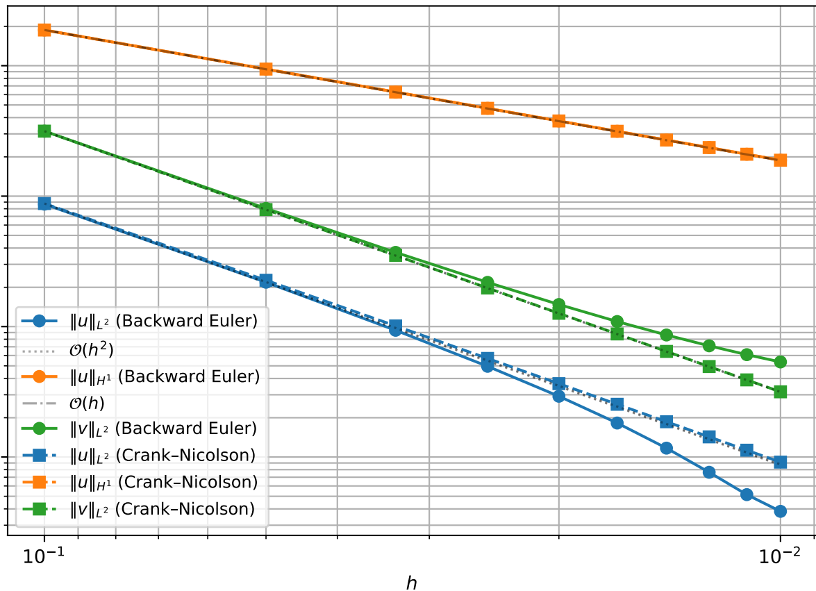
Spatial convergence comparison ( \Delta t = 0.01 )
