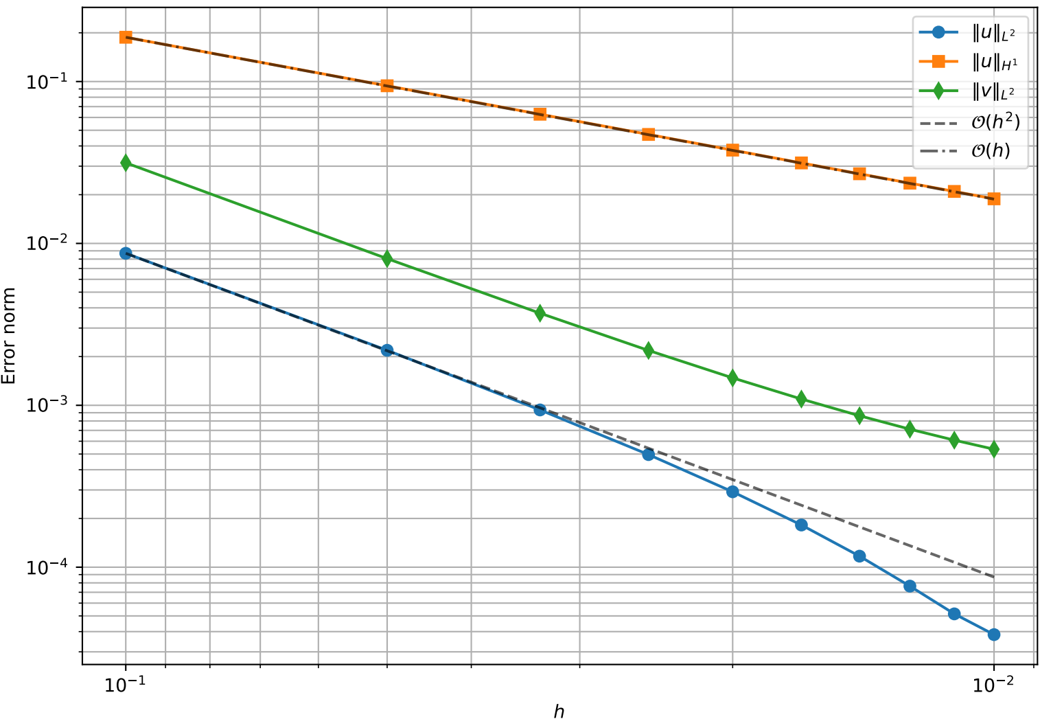
Spatial convergence (Backward Euler, T = 1 )
