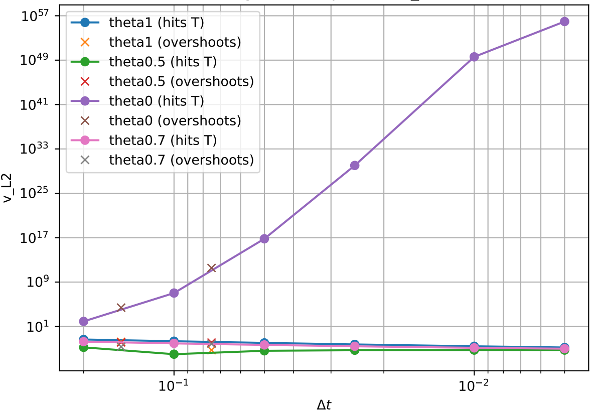
Time convergence comparison: v_{L2} at t = T
