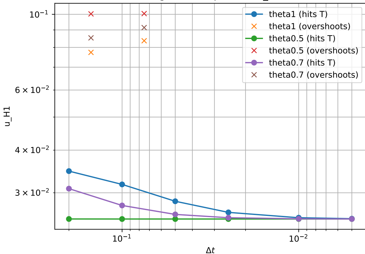
Time convergence comparison: u_{H1} at t = T
