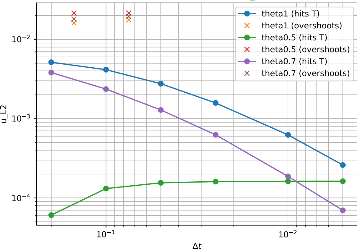
Time convergence comparison: u_{L2} at t = T
