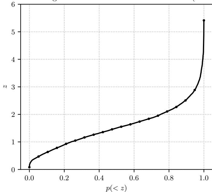
SDSS catalogue: inverse cumulative distribution (redshift)
