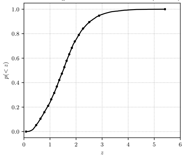
SDSS catalogue: inverse cumulative distribution (redshift)
