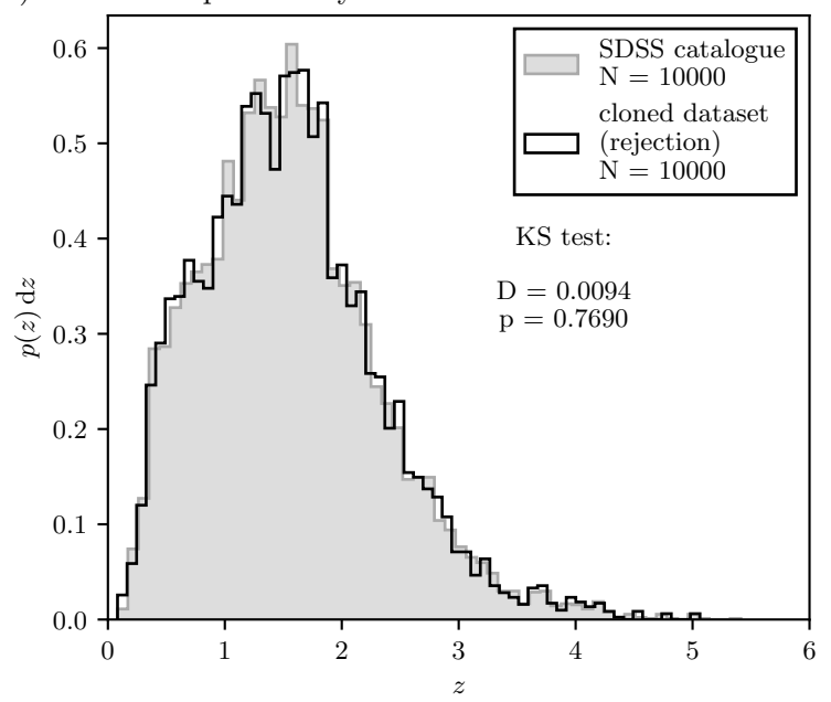
Redshift probability distribution: measured and cloned
