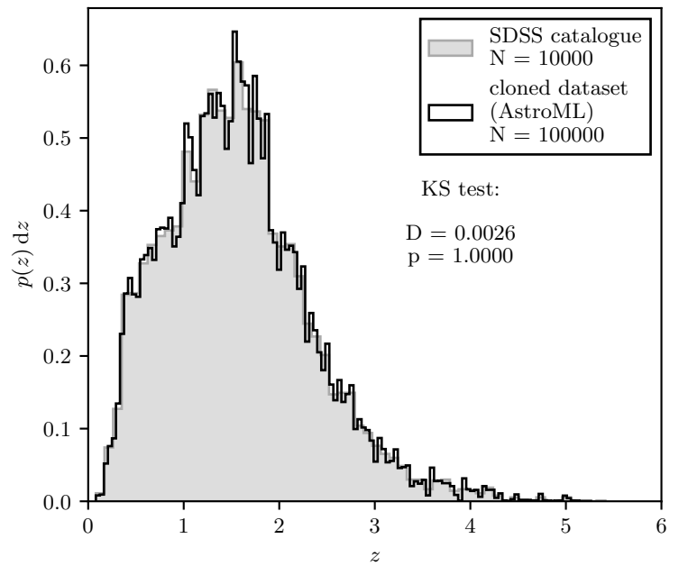
Redshift probability distribution: measured and cloned
