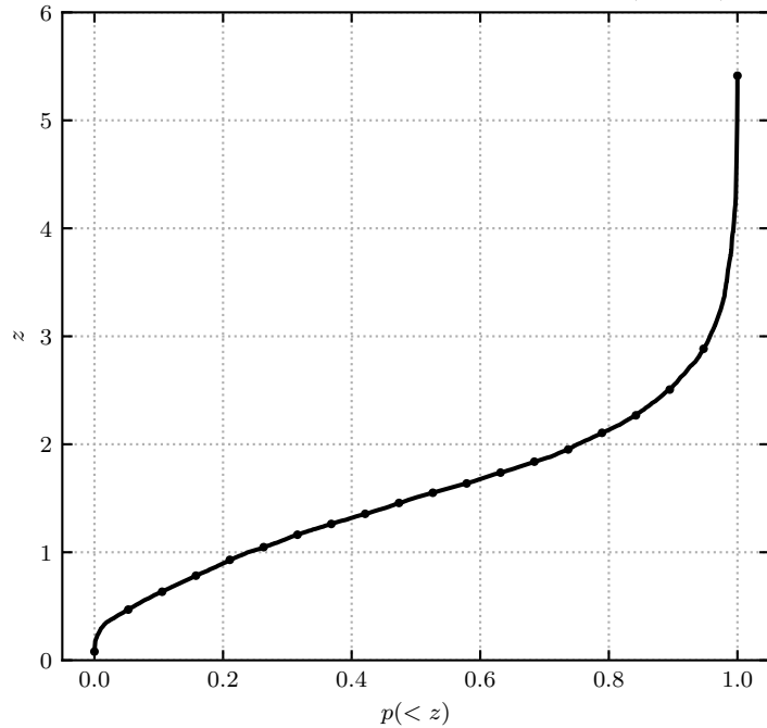
SDSS catalogue: inverse cumulative distribution (redshift)
