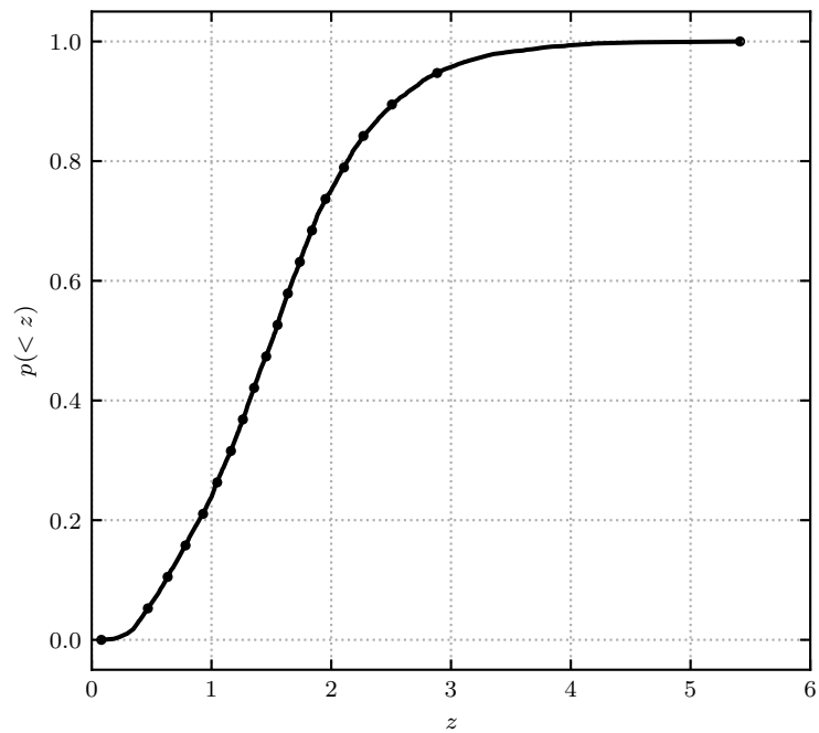
Redshift probability distribution: measured and cloned
