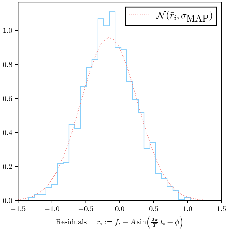
Residual after sinusoid MCMC fit
