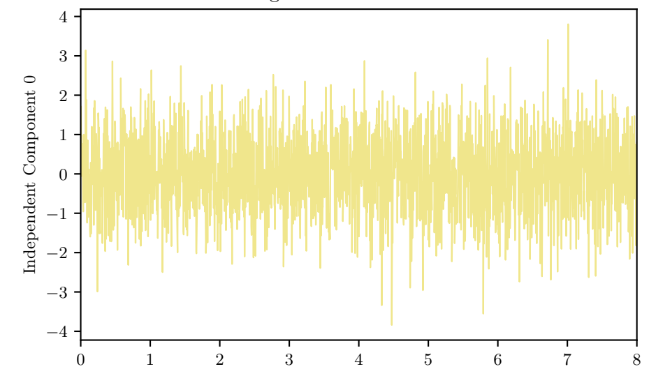
Signals in the ICA basis
