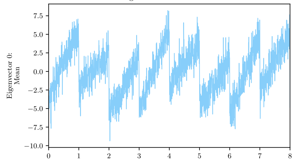
Signals in the PCA basis
