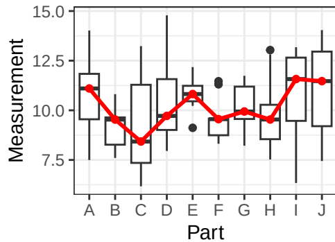
\bar{x} Chart
