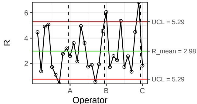
R Chart
