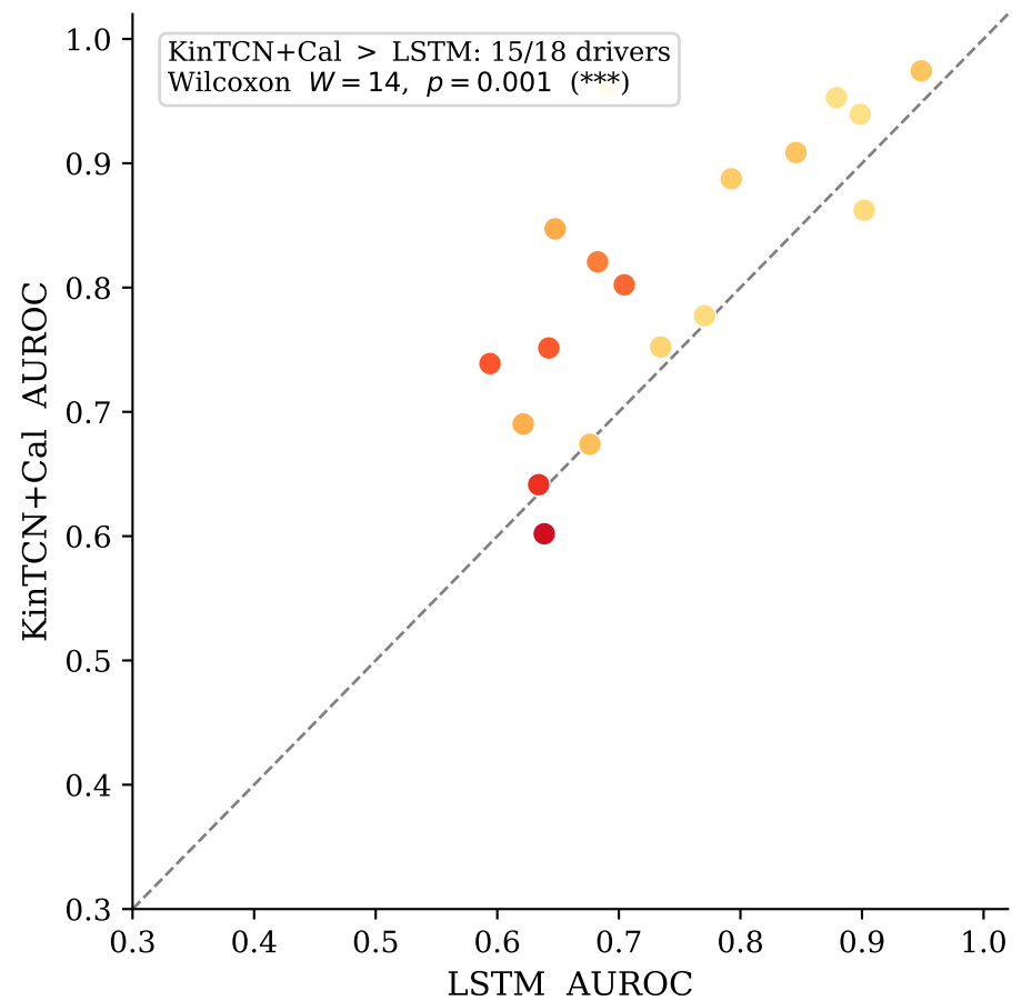
Per-driver AUROC ( L = 45 \sim s , H = 10 \sim s )
