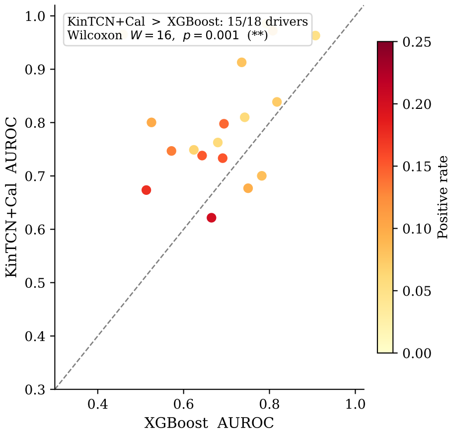
Per-driver AUROC ( L = 45 \sim s , H = 10 \sim s )
