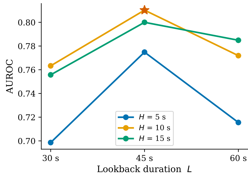
(a) Discrimination
