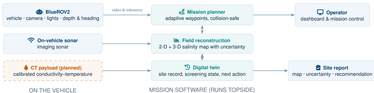
Figure 3: System overview. Solid blue vehicle panels: hardware owned today. Dashed panel: the planned calibrated CT sensor. Teal panels: mission software already implemented and exercised in simulation.
