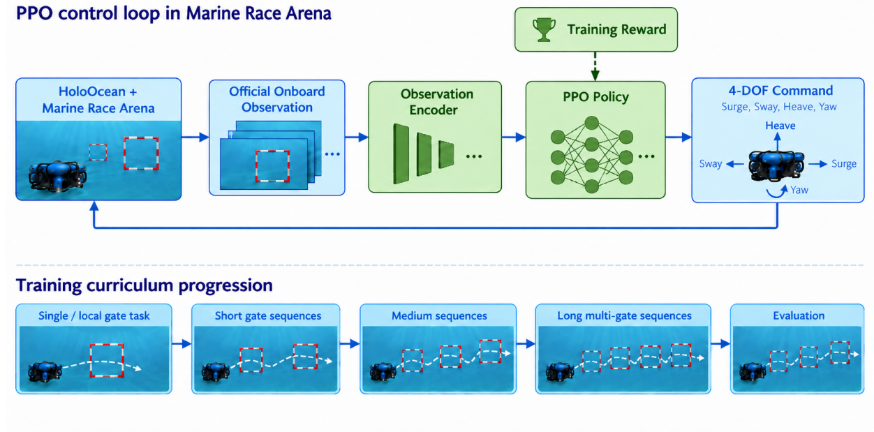
Figure 15: Gen-2 recurrent-policy loop and curriculum.
