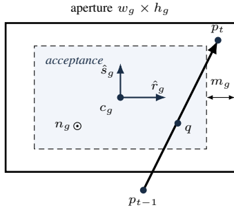
Fig. 3. Gate-crossing validation. A valid crossing pierces the gate plane in the normal direction ((13)) at a point q ((14)) inside the aperture shrunk on every side by the safety margin m_g ((15)); the frame (\hat{r}_g, \hat{s}_g, n_g) follows the passage direction.
