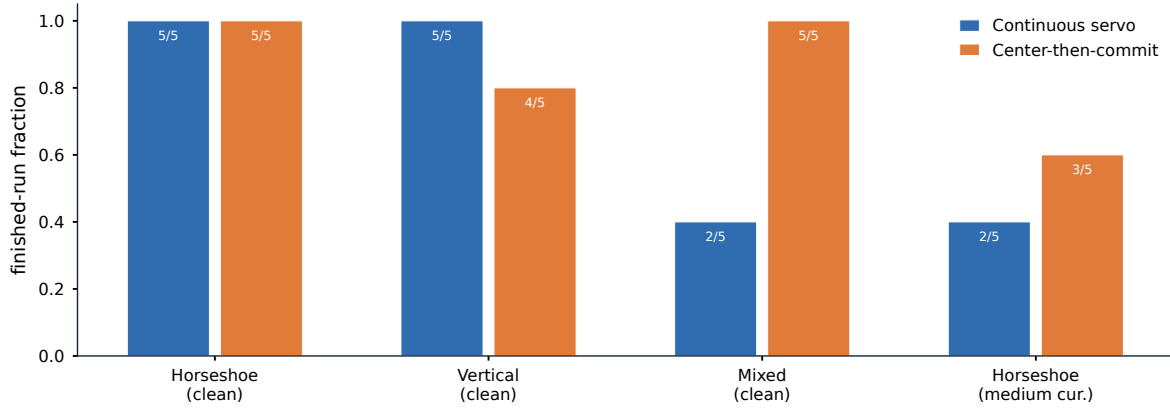
Figure 16: Reference-controller completion on clean and medium-current conditions.
