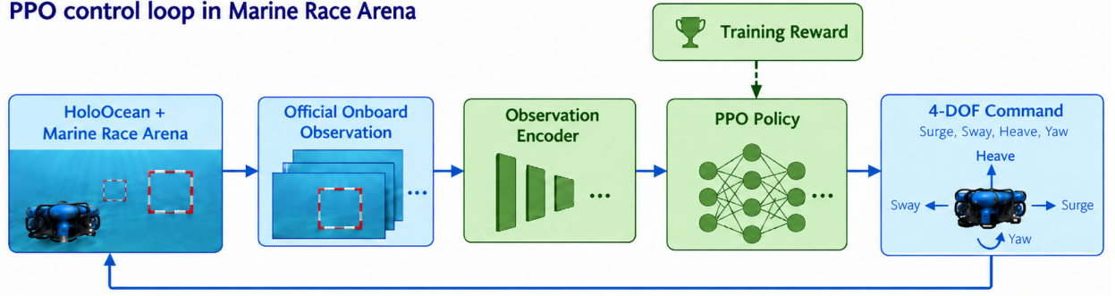
Figure 15: Control loop of the recurrent learning-based controller. The official onboard observation is encoded and consumed by the policy, which returns the same four-degree-of-freedom body-frame command as any other participant, while the training reward acts only during training and never enters the observation.
