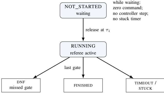
Fig. 4. Participant lifecycle. A rover is released to RUNNING at its start delay \tau_i (a single rover is the case \tau_i = 0 ) and reaches a terminal state by finishing, missing a gate (DNF) or timing out.
