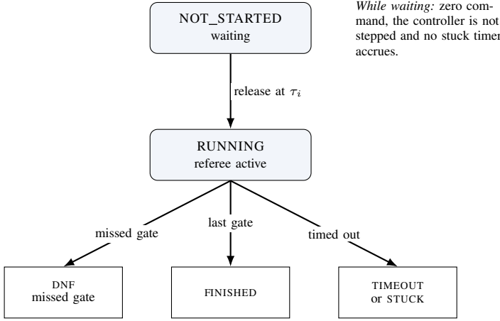
Fig. 4. Participant lifecycle. A rover is released to RUNNING at its start delay \tau_i (a single rover is the case \tau_i = 0 ) and reaches a terminal state by finishing, missing a gate (DNF) or timing out.
