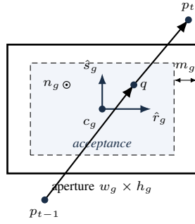
Fig. 3. Gate-crossing validation. A valid crossing pierces the gate plane in the normal direction ((13)) at a point q ((14)) inside the aperture shrunk on every side by the safety margin m_g ((15)); the frame (\hat{r}_g, \hat{s}_g, n_g) follows the passage direction.
