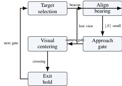
Fig. 2. Simplified state logic of the rule-based baseline: target selection, bearing alignment, gate approach, visual centering and exit hold before advancing to the next gate.
