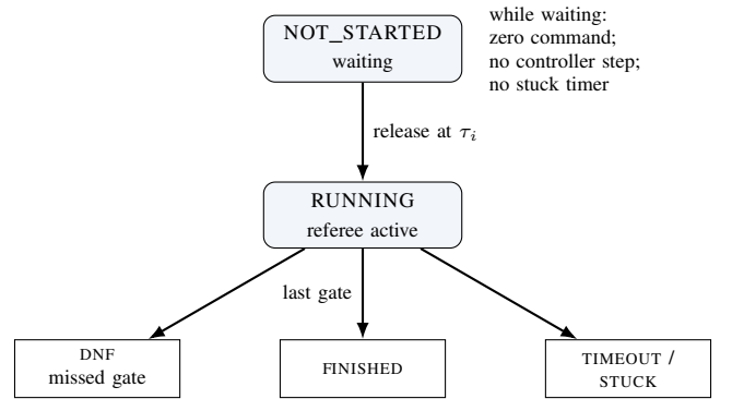
Fig. 3. Participant lifecycle. A rover is released to RUNNING when the clock reaches its start delay \tau_i ; before release it receives a zero command, its controller is not stepped and no stuck or gate-timeout timer accrues. Running rovers reach a terminal state by finishing the last gate, missing a gate (DNF) or exceeding a timeout/stuck condition. A single-rover run is the degenerate case \tau_i = 0 .
