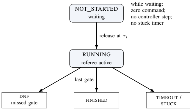
Fig. 3. Participant lifecycle. A rover is released to RUNNING when the clock reaches its start delay \tau_i ; before release it receives a zero command, its controller is not stepped, and no stuck or gate-timeout timer accrues. Running rovers reach a terminal state by finishing the last gate, missing a gate (DNF), or exceeding a timeout/stuck condition. A single-rover run is the degenerate case \tau_i = 0 .
