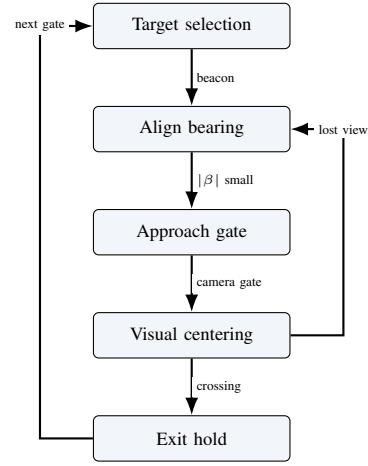
Fig. 2. Rule-based controller states from target selection to gate exit.
