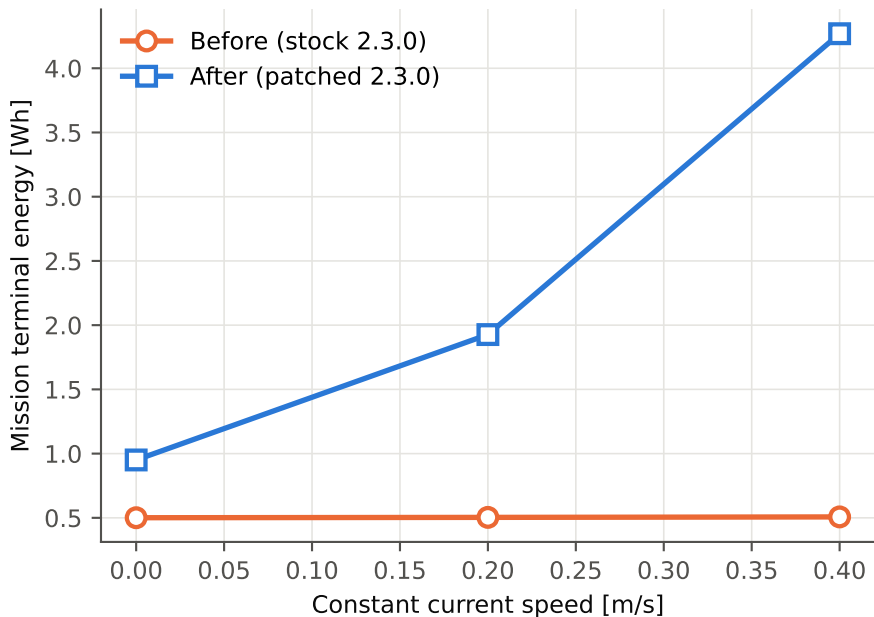
D. Transit-yaw-return mission: current vs energy
