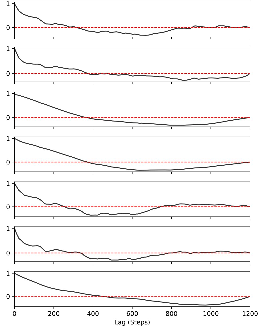
Autocorrelation Function
