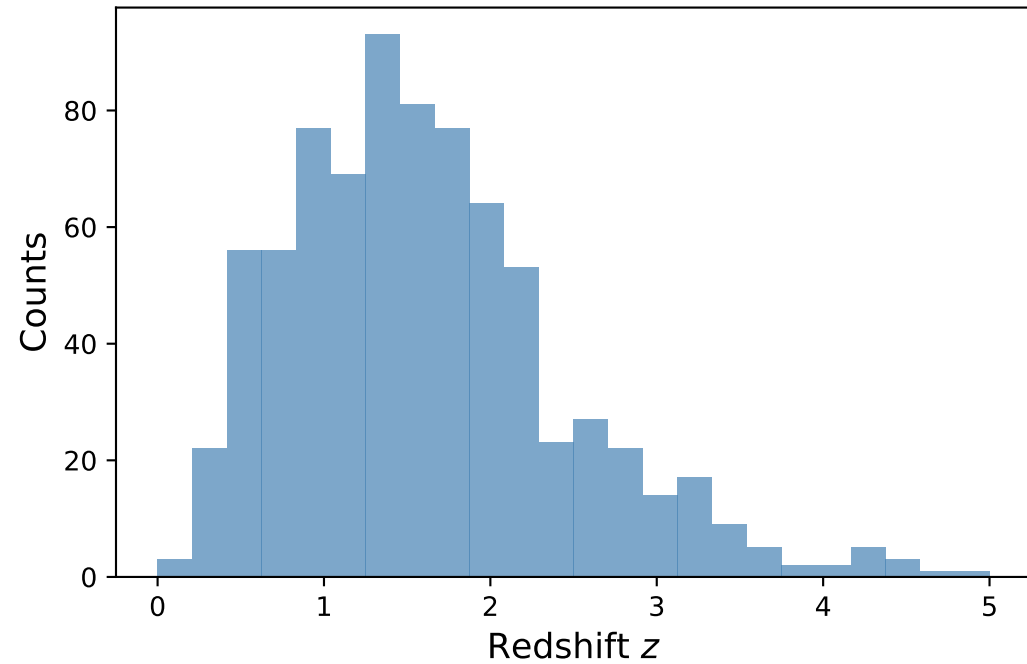
Detected Redshifts (10 yr)
