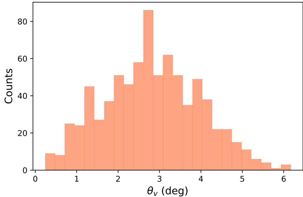
Detected Viewing Angles (10 yr)
