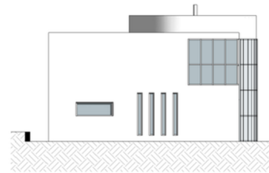
North elevation
