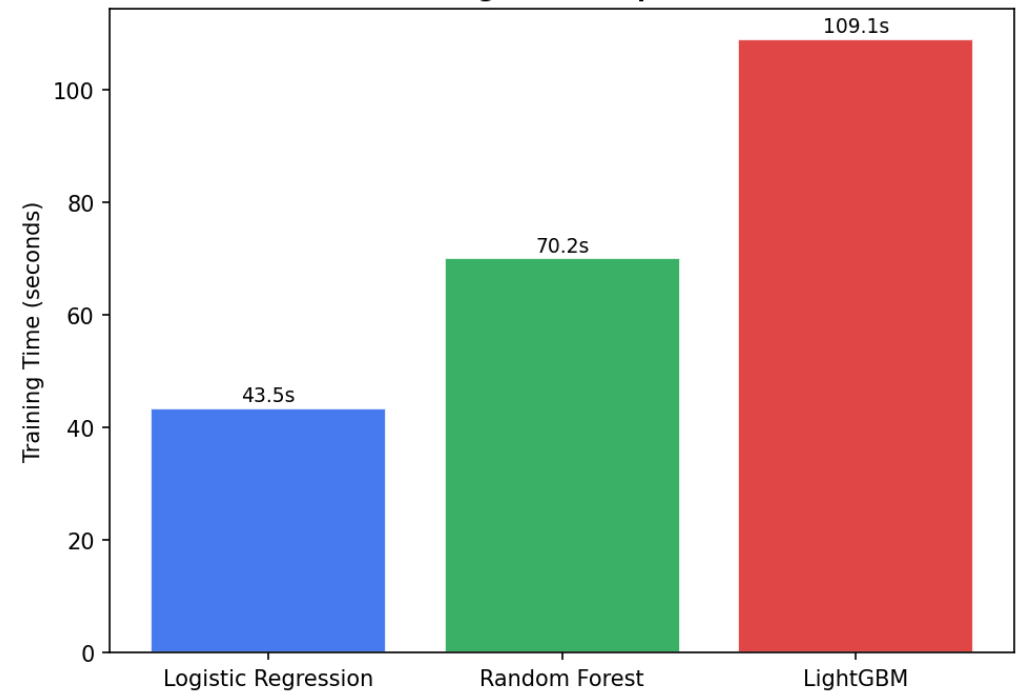
Training Time Comparison
