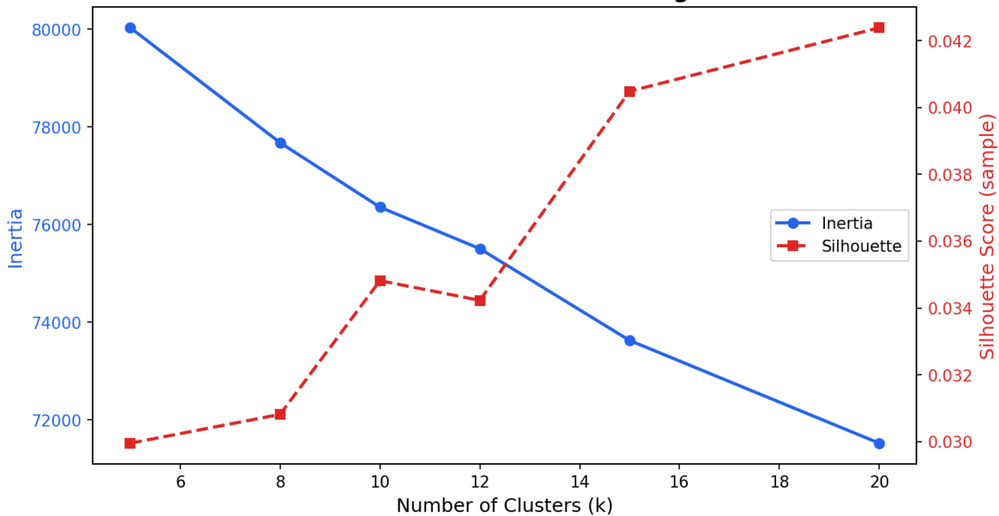
Elbow & Silhouette — Choosing k
