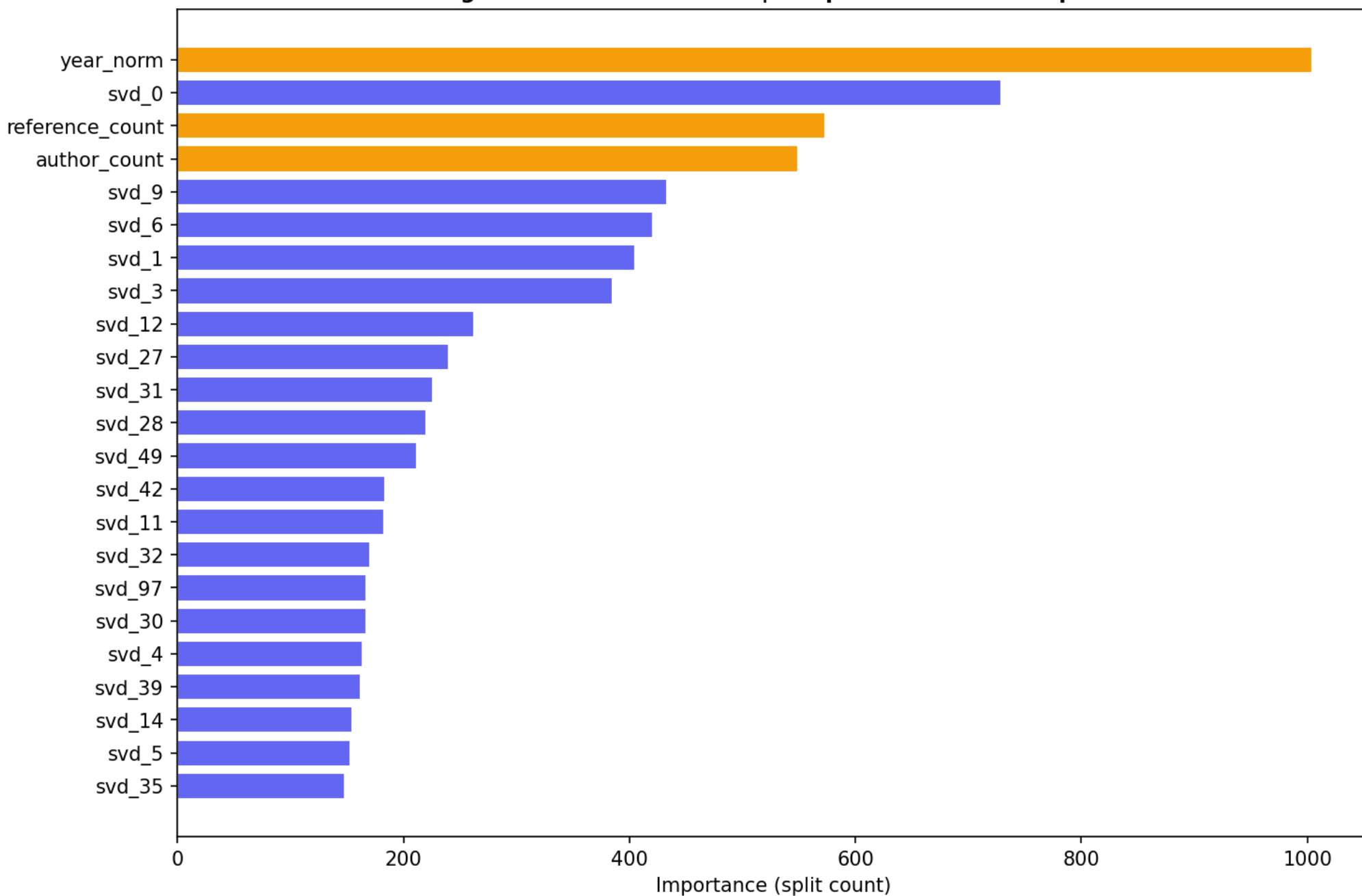
LightGBM Feature Importance (top 23) Orange = structured feature | Purple = SVD text component
