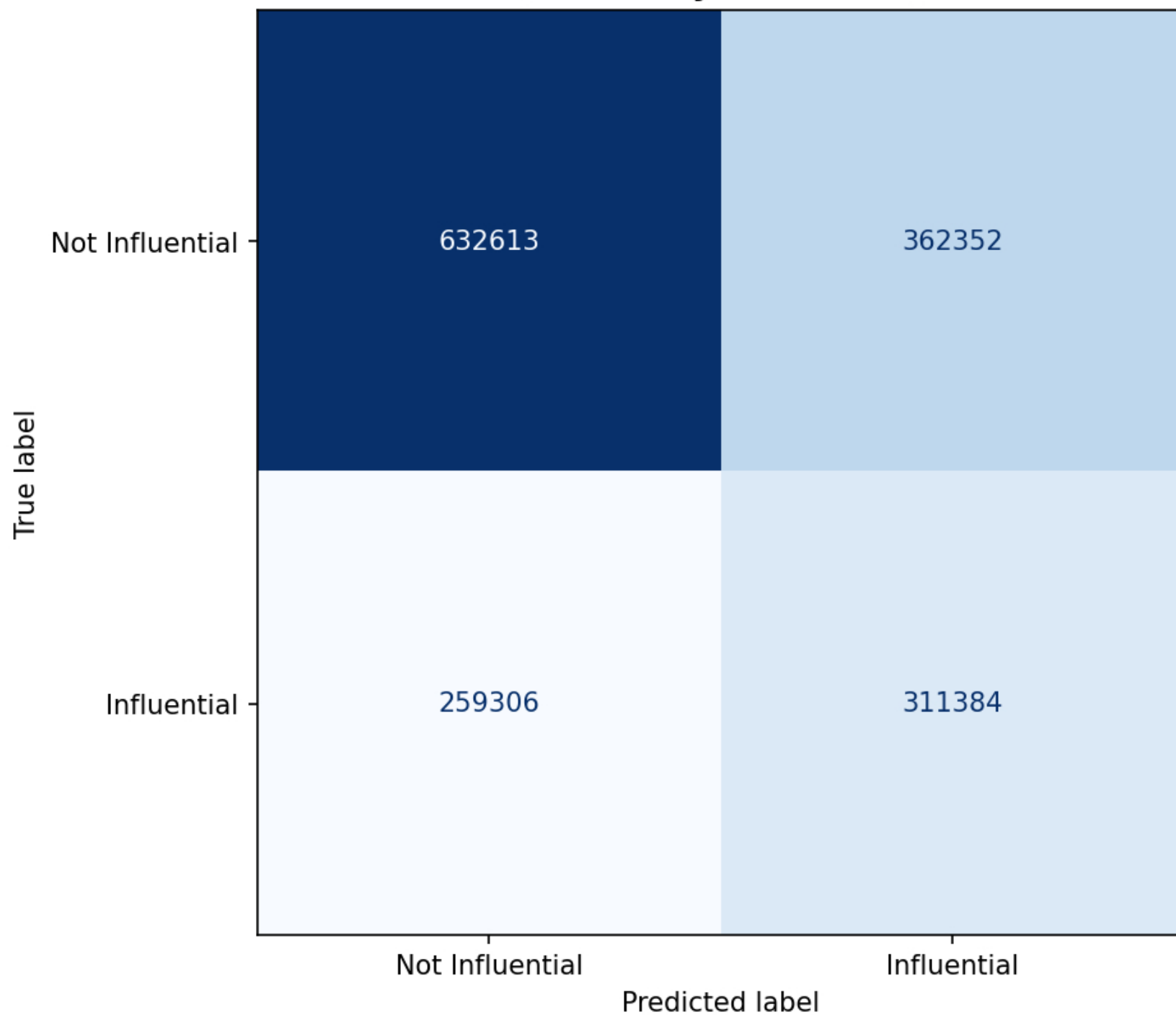
Confusion Matrix — LightGBM (test set: year \geq 2010)
