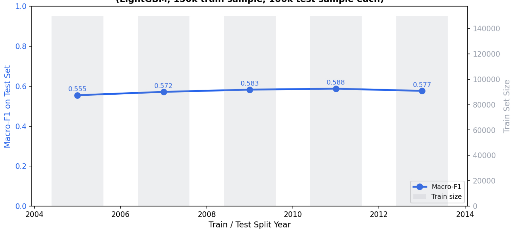
Model Performance vs. Train/Test Year Threshold (LightGBM, 150k train sample, 100k test sample each)
