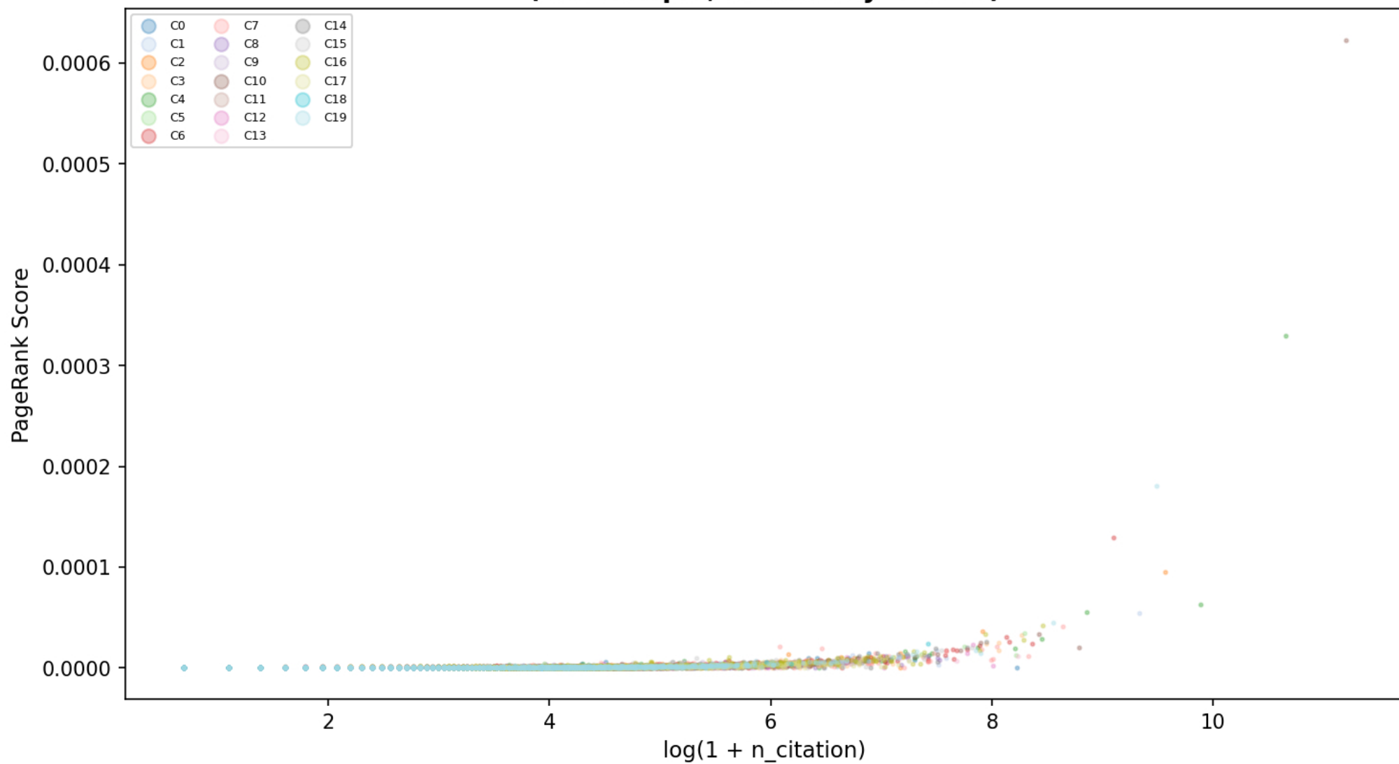
PageRank vs Citation Count (80k sample, colored by cluster)
