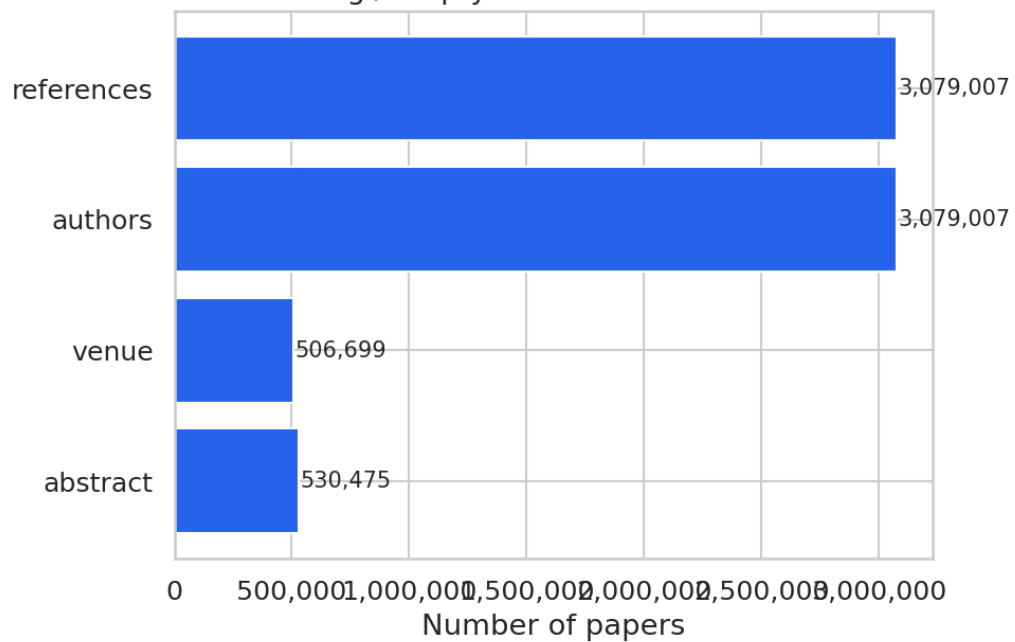
Missing / Empty Fields — Absolute Count
