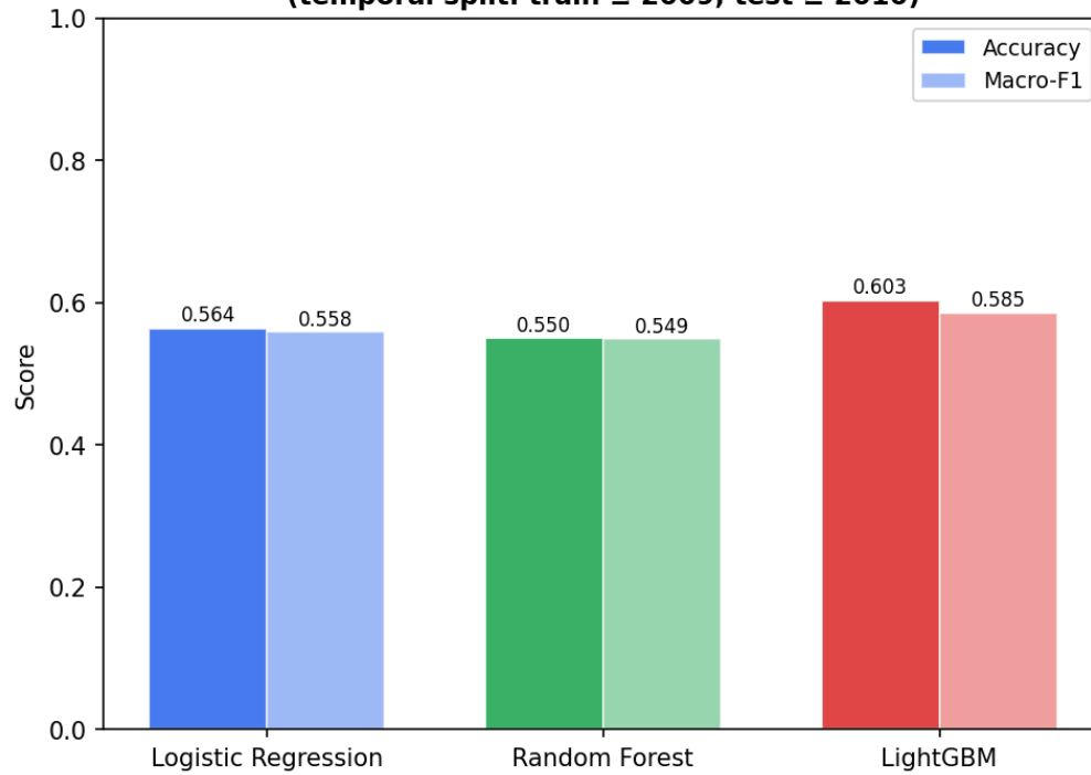
Model Accuracy & Macro-F1 (temporal split: train \leq 2009, test \geq 2010)
