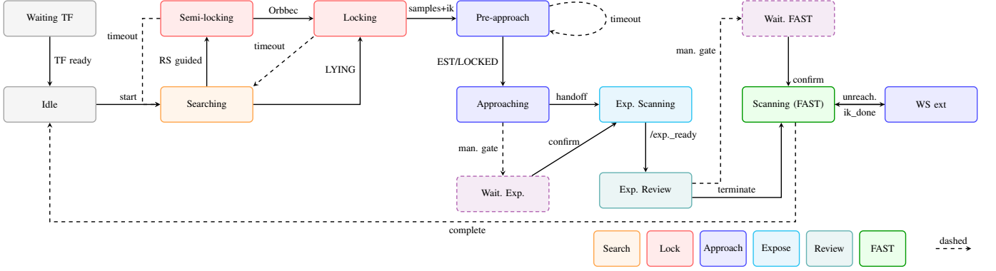
Fig. 2. Mission FSM with 13 states. The robot searches for the patient through body rotation and dual-sensor confirmation (SEARCHING → SEMI_LOCKING → LOCKING), approaches while running the anticipatory scanner (PRE_APPROACH → APPROACHING), performs a posture-adaptive exposure body scan with integrated wound and burn detection (EXPOSURE_SCANNING), enters an interactive review phase for operator-driven re-inspection (EXPOSURE_REVIEW), and executes FAST ultrasound scanning with pre-planned body reconfiguration (SCANNING). Transitions are triggered by perception confidence (dashed) or geometric conditions (solid).
