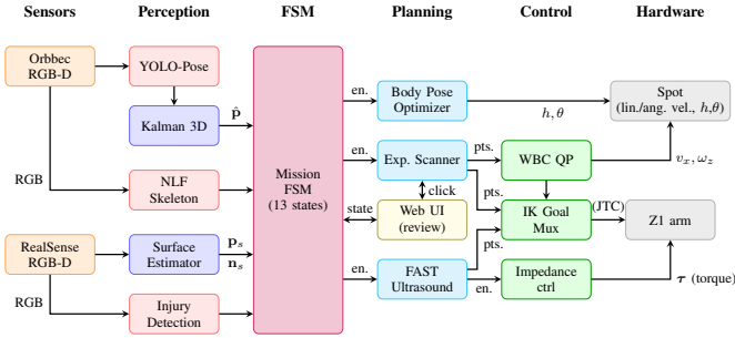
Fig. 3. System block diagram. The Perception layer processes dual-sensor RGBD streams via YOLO-pose, Kalman filtering, NLF! skeleton detection, surface estimation, and injury detection. The 13-state Mission FSM orchestrates four Planning modules: Exposure Scanner, FAST Ultrasound, Body Pose Optimizer, and the Web UI for interactive review. The Control layer executes real-time decisions through the WBC QP, IK Goal Multiplexer, and Impedance Controller. Dashed arrows denote operator-triggered or posture-optimisation paths.
