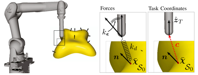
Fig. 1. Target surface and task coordinates of our impedance controller. Each point on the surface S_0 can be assigned a unique, directed normal vector (left). The task coordinates result in a wrench pulling the tool to the surface and orienting it along the surface normal (middle). Calculation of the coordinates is based on the proxy point \bar{\chi} \in S_0 on the surface, the corresponding surface normal n and the vector c between \bar{\chi} and tool position x_t .
