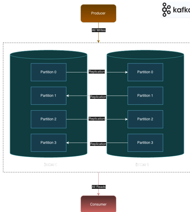
Figura 2. Kafka Cluster
