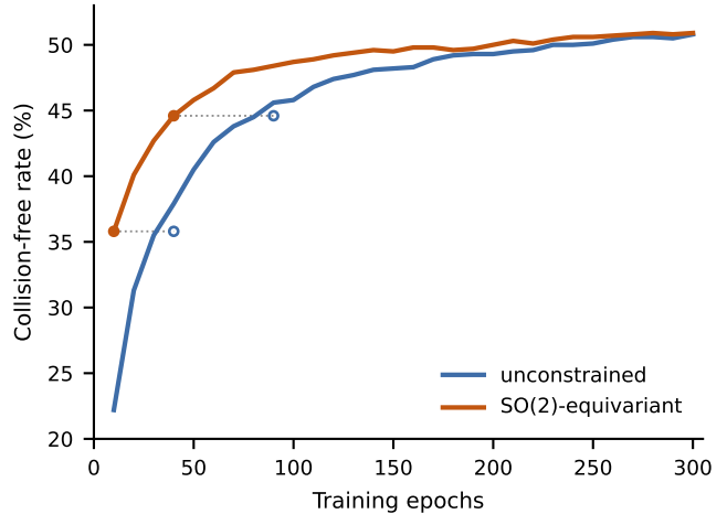
Figure 5. The constraint buys optimisation, not accuracy. Both arms converge to the same held-out rate; the equivariant one arrives roughly four times sooner. Dotted lines mark where the unconstrained arm first reaches the equivariant arm’s epoch-10 and epoch-40 values. Seed 0 at 60 environments; the seed-matched difference at epoch 300 is +0.15 points.
