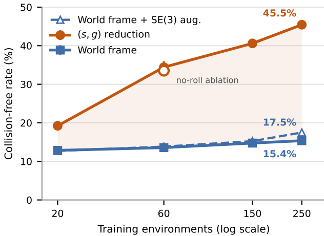
Figure 3. The gap widens with data. If canonicalisation were compensating for a shortage of training data one would expect it to close; instead the world-frame baseline is nearly flat while the reduced model continues to improve. The hollow marker is the no-roll ablation, drawn on the treatment line because it is the same arm with one component removed
