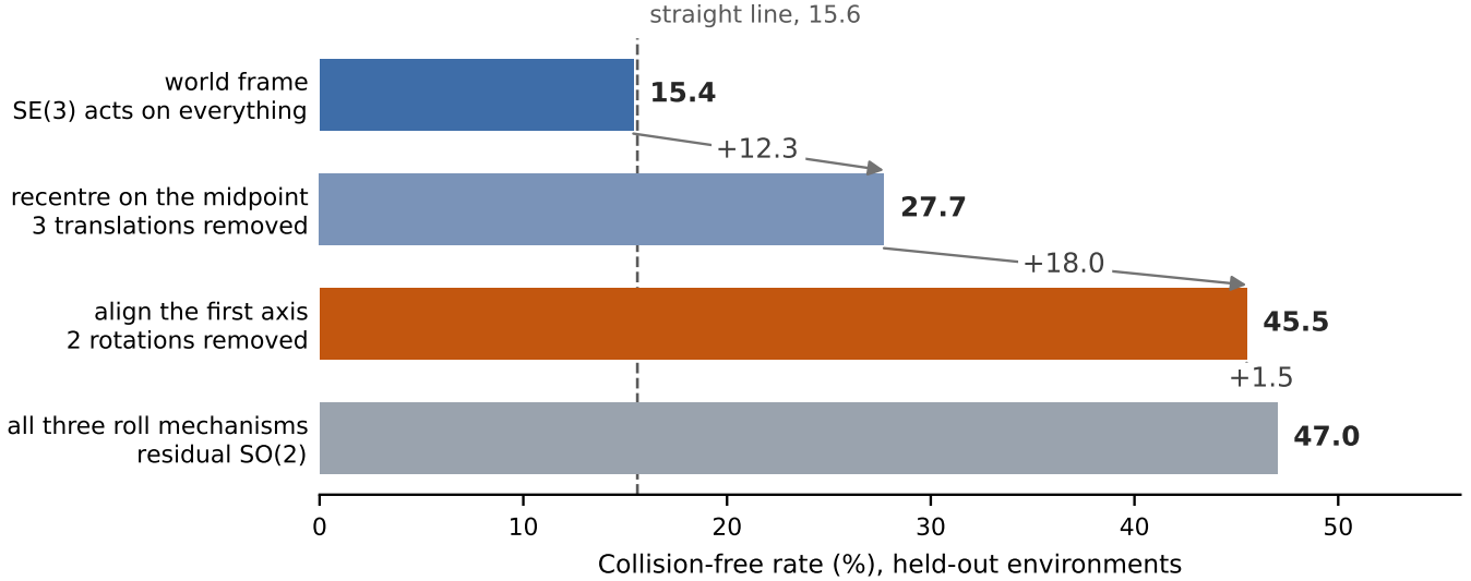
Figure 2. SE(3) taken apart one stage at a time, at 250 training environments. Every bar is a measured arm rather than a term in a decomposition: the second is a translation-only reduction, trained and evaluated like the others. The increments between them are what each group of degrees of freedom is worth. The bottom bar adds all three mechanisms built for the residual SO(2) — roll augmentation, frame averaging and an equivariant backbone — and is deliberately drawn on the same scale: its near-coincidence with the bar above is the paper’s second finding. The dashed line is a straight segment from start to goal on the identical problems, which the world-frame arm does not beat.
