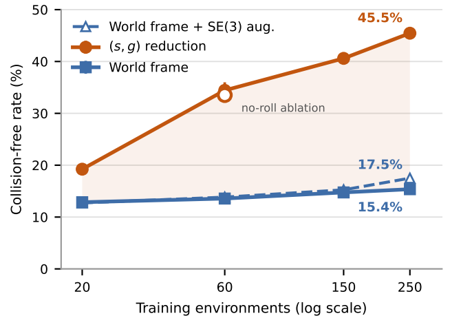
Figure 3. The gap widens with data. If canonicalisation were compensating for a shortage of training data one would expect it to close; instead the world-frame baseline is nearly flat while the reduced model continues to improve. The hollow marker is the no-roll ablation, drawn on the treatment line because it is the same arm with one component removed
