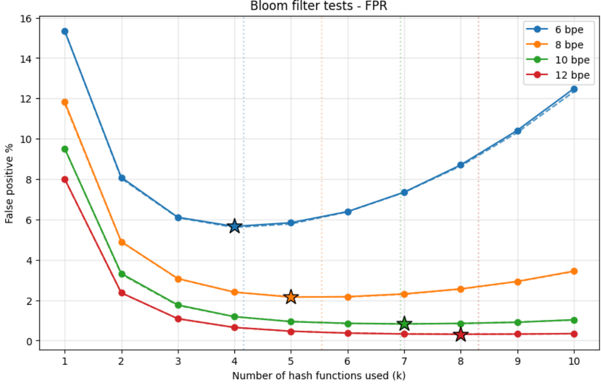
Figure 1: Bloom filter behavior with when tested with a 10.0 fake IDs proportion
