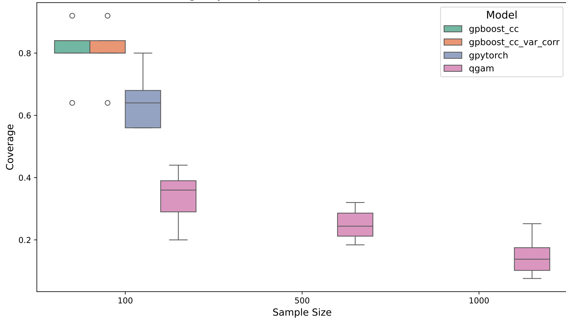
coverage by Sample Size. Likelihood: ald. Dim: 1
