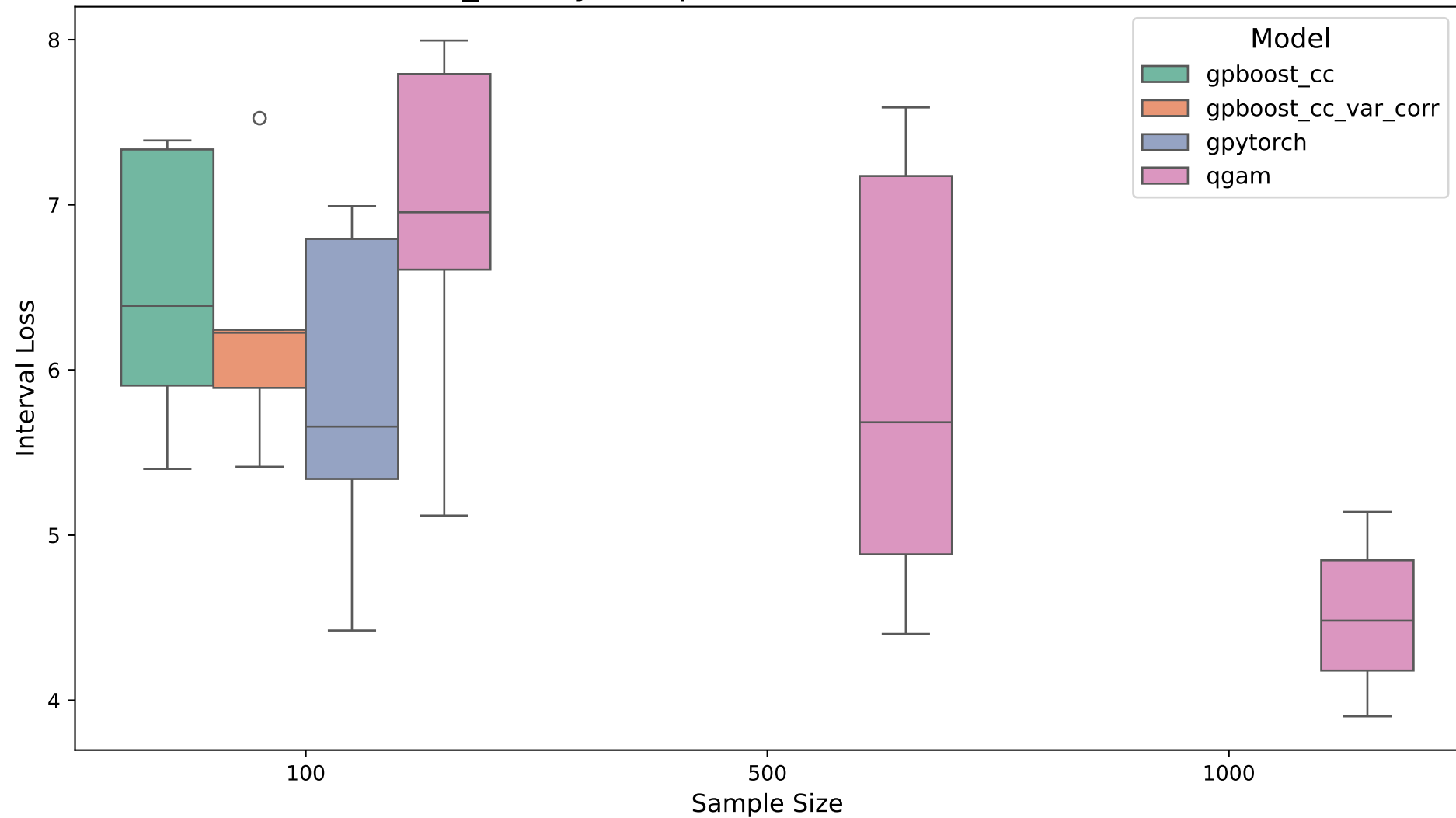
interval_loss by Sample Size. Likelihood: ald. Dim: 3
