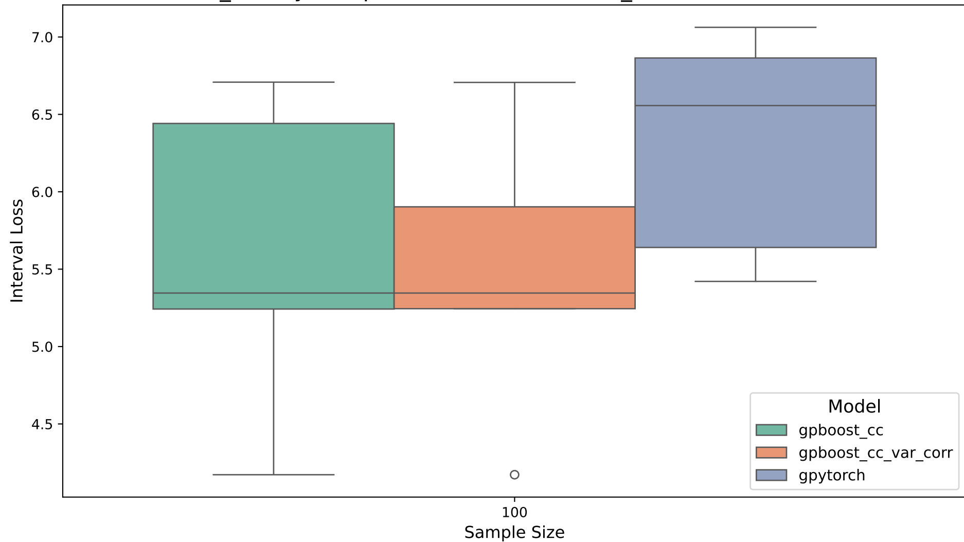
interval_loss by Sample Size. Likelihood: ald_heteroscedastic. Dim: 3
