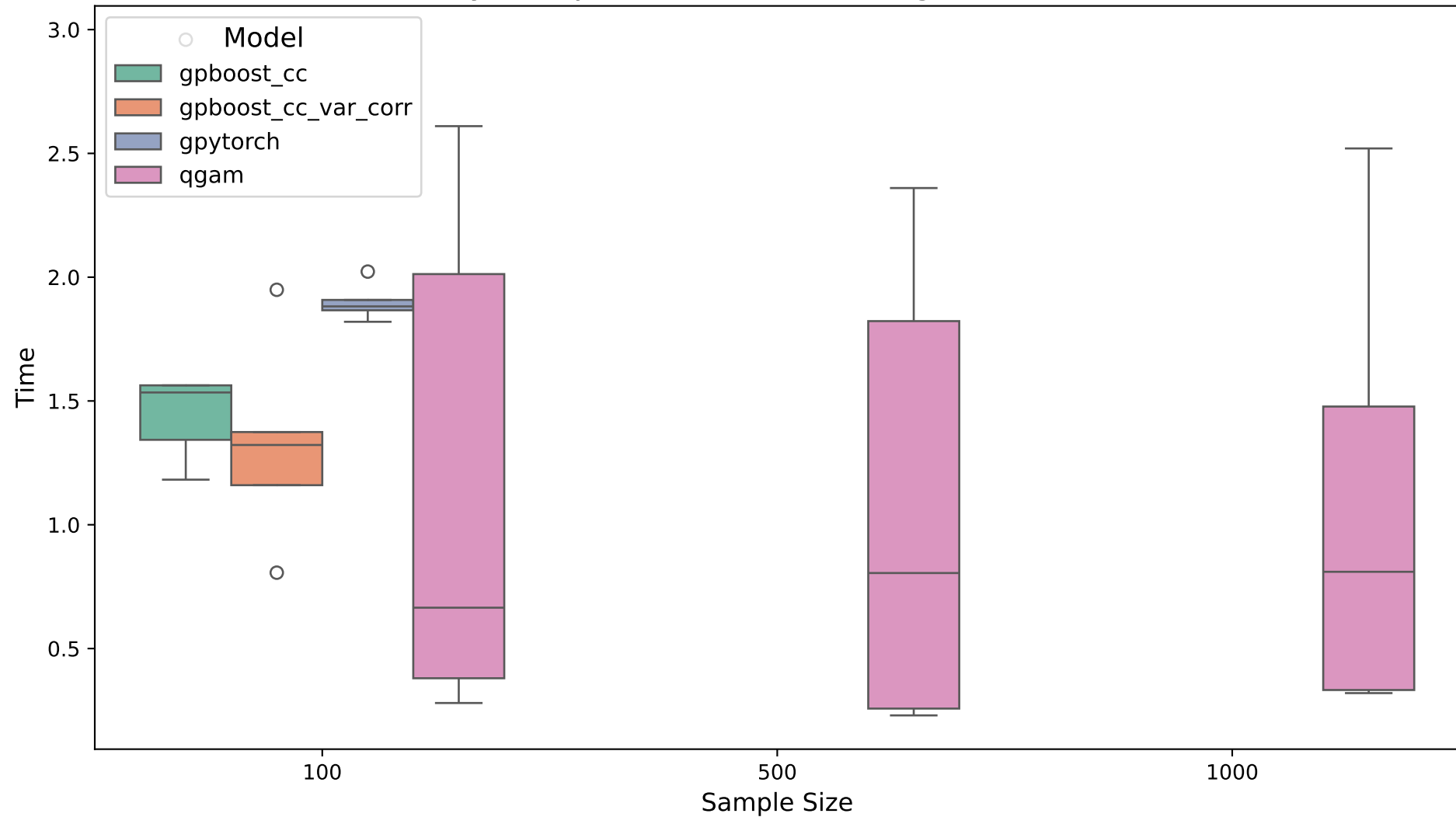
time by Sample Size. Likelihood: gaussian. Dim: 3
