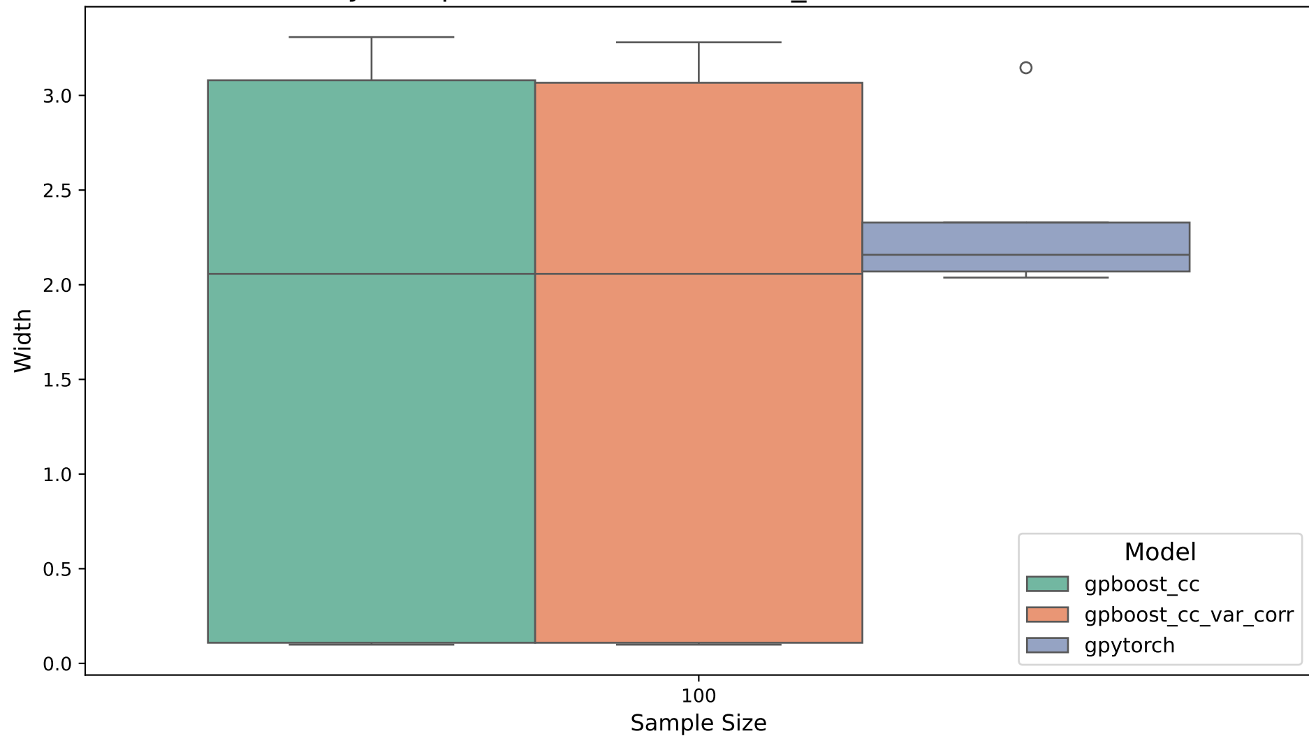
width by Sample Size. Likelihood: ald_heteroscedastic. Dim: 2
