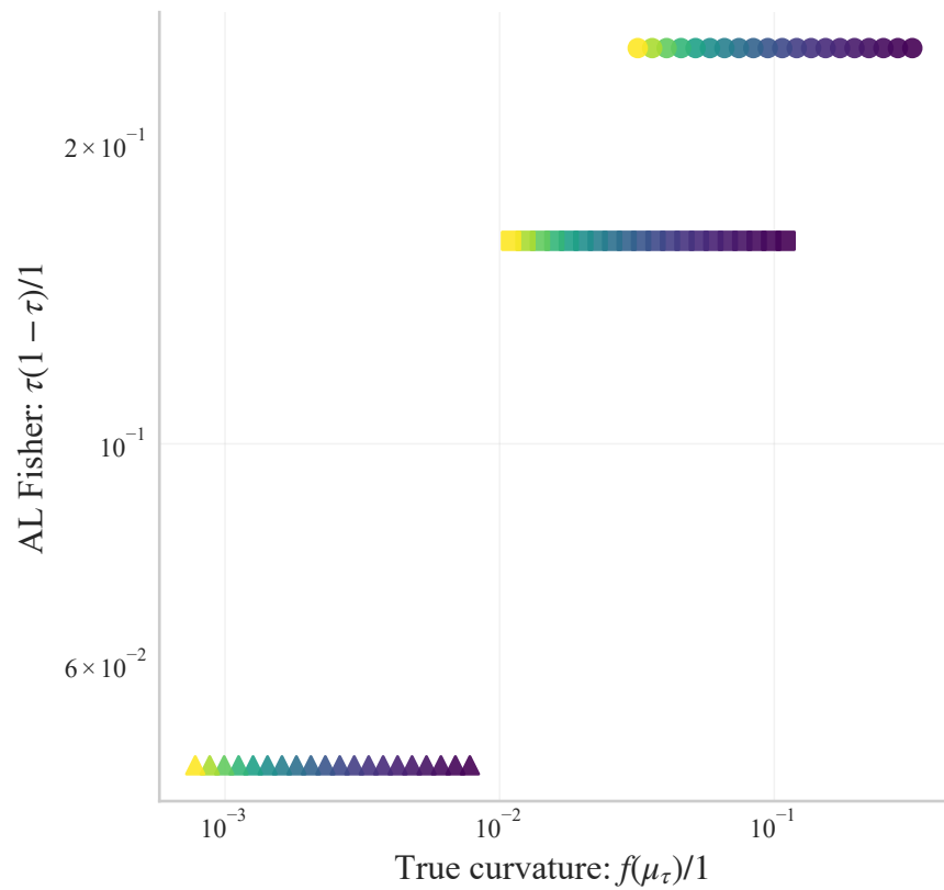
Scale fixed to \lambda = 1
