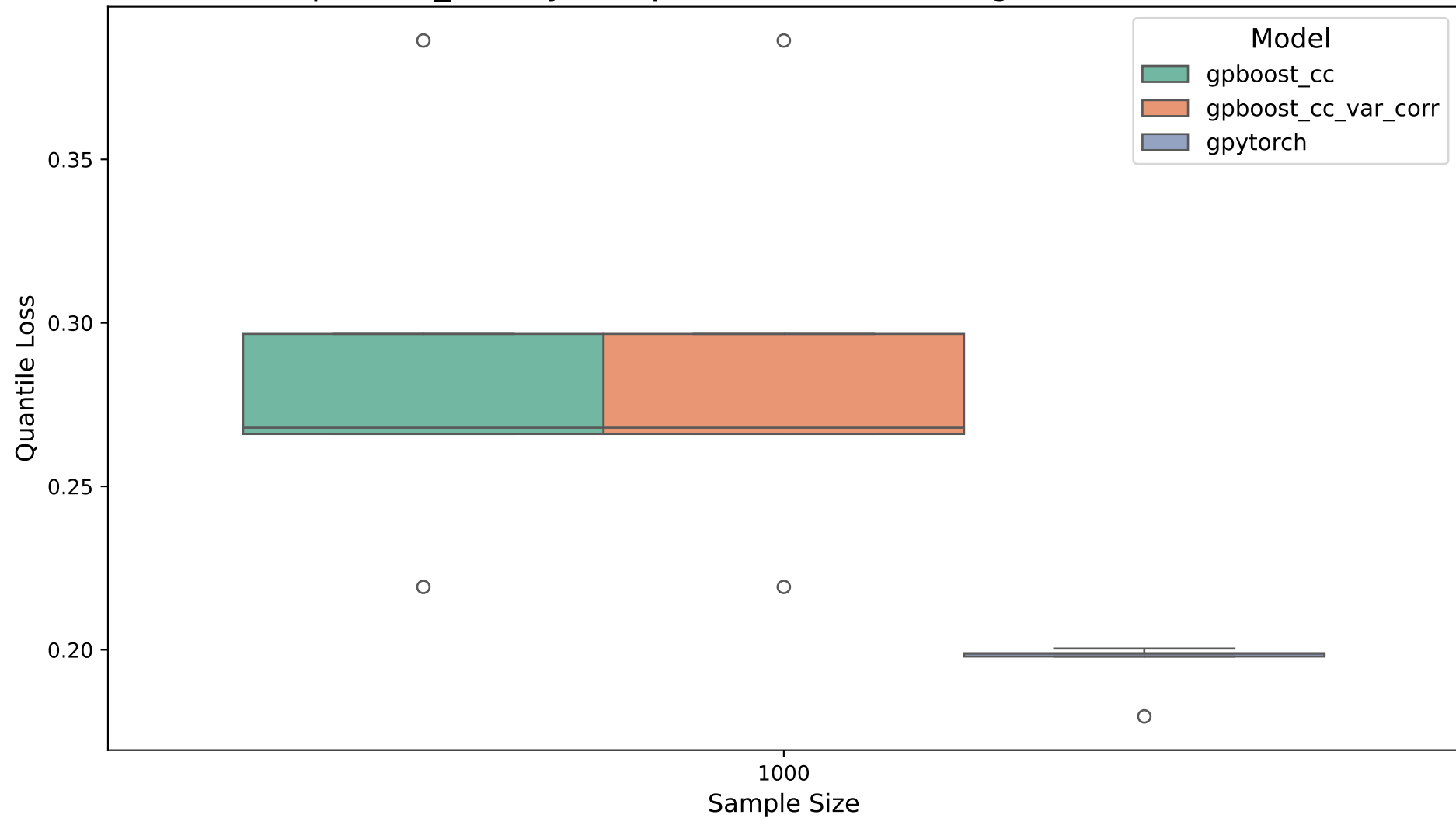
quantile_loss by Sample Size. Likelihood: gaussian. Dim: 3
