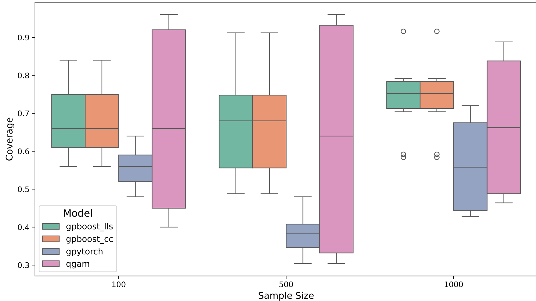
coverage by Sample Size. Likelihood: gaussian. Dim: 2
