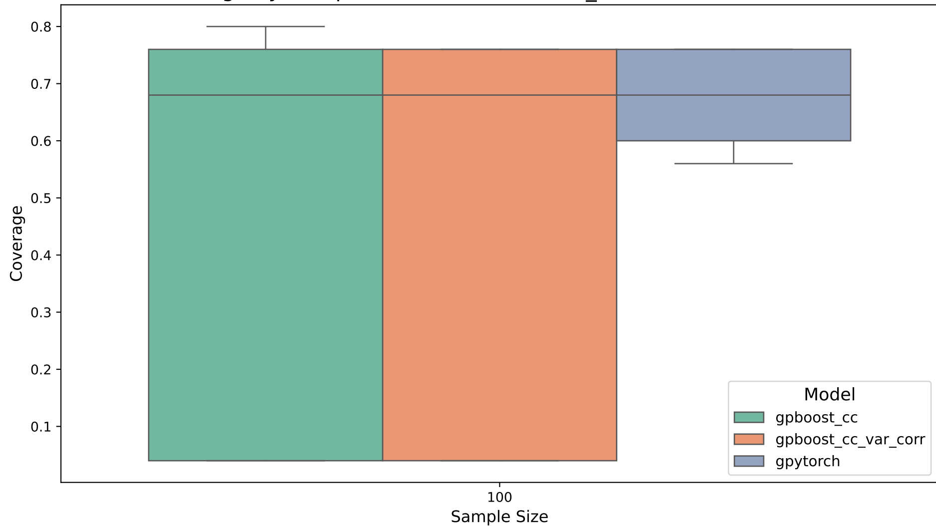
coverage by Sample Size. Likelihood: ald_heteroscedastic. Dim: 1
