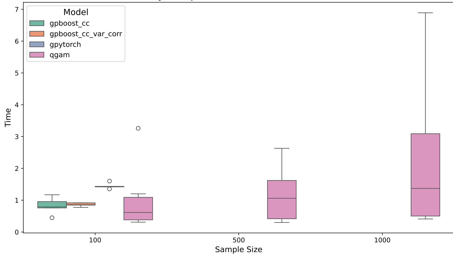
time by Sample Size. Likelihood: ald. Dim: 3
