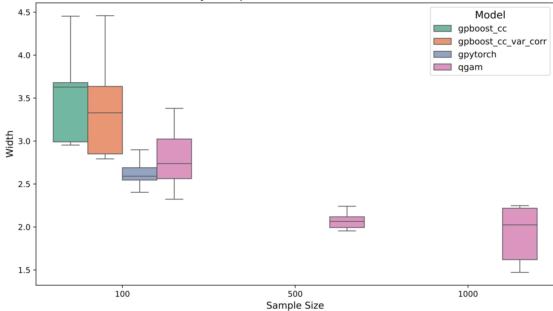
width by Sample Size. Likelihood: ald. Dim: 2
