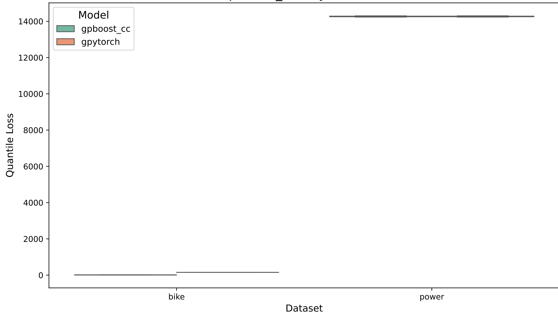
quantile_loss by Dataset.
