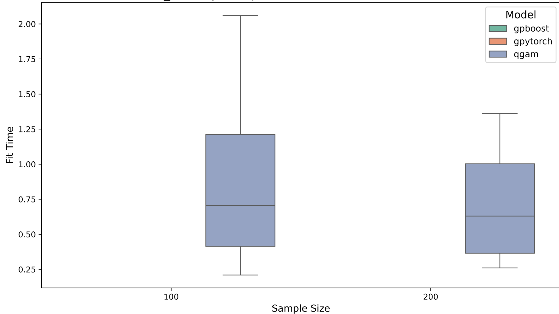
fit_time by Sample Size. Likelihood: ald. Dim: 2
