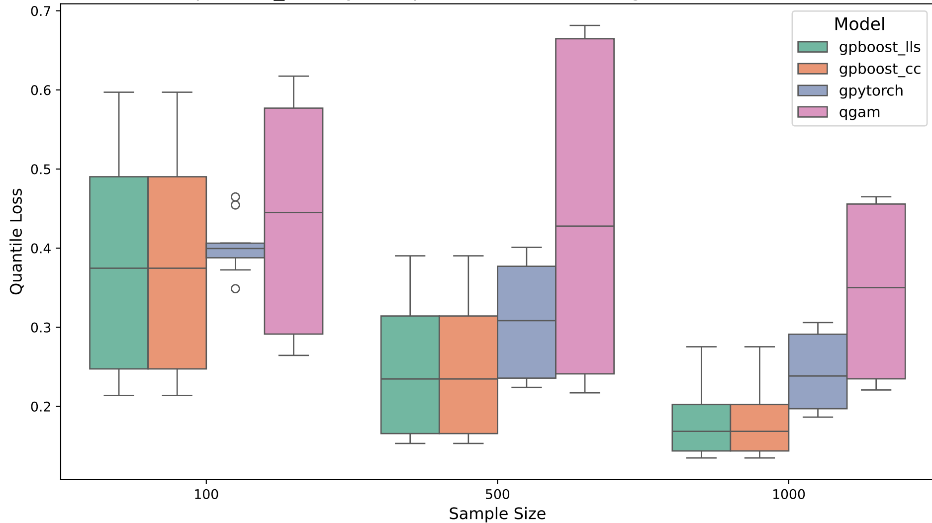
quantile_loss by Sample Size. Likelihood: gaussian. Dim: 1
