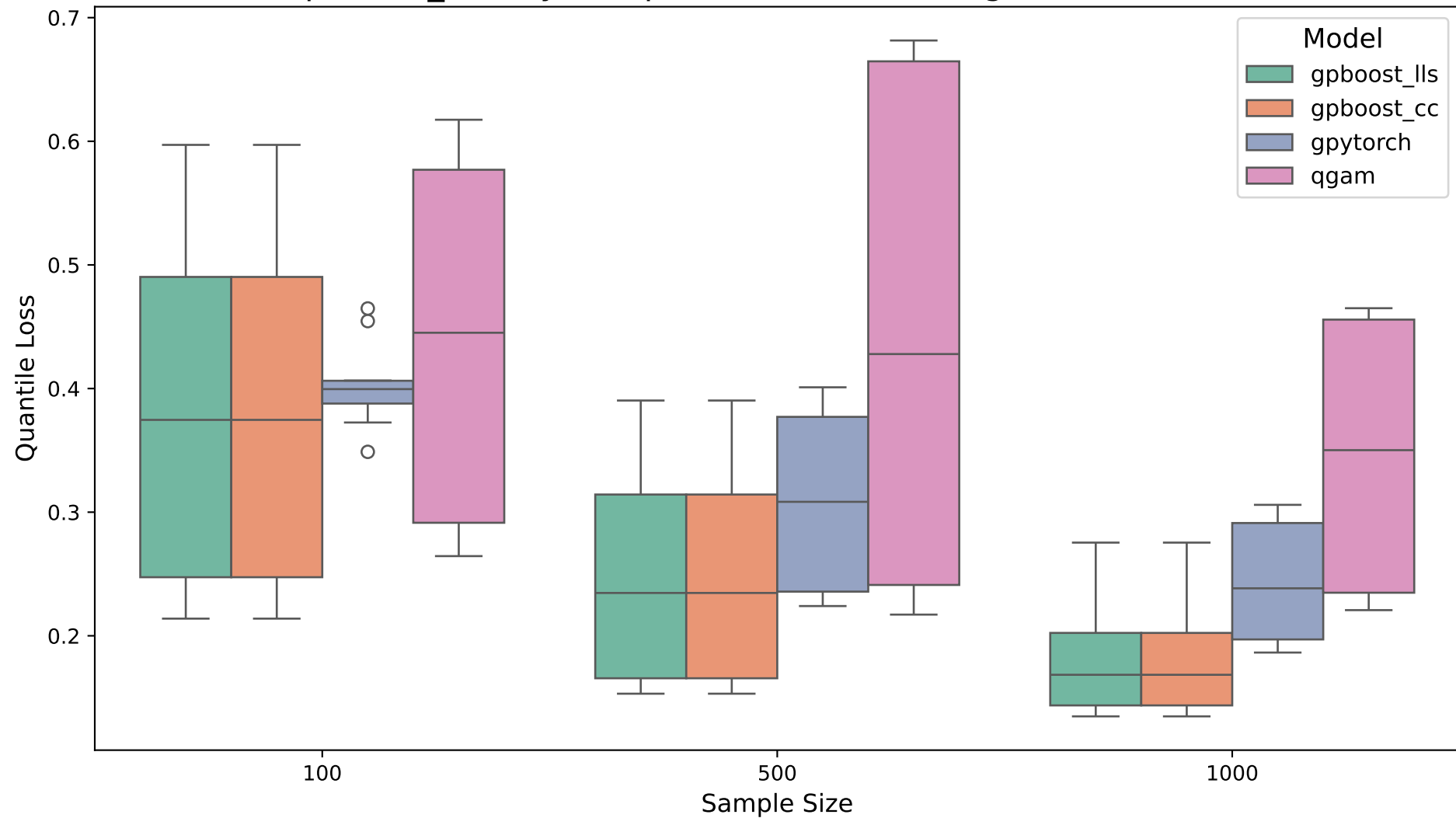
quantile_loss by Sample Size. Likelihood: gaussian. Dim: 2
