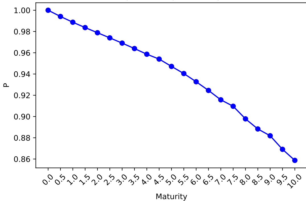
Zero coupon bond price, range [0,10]
