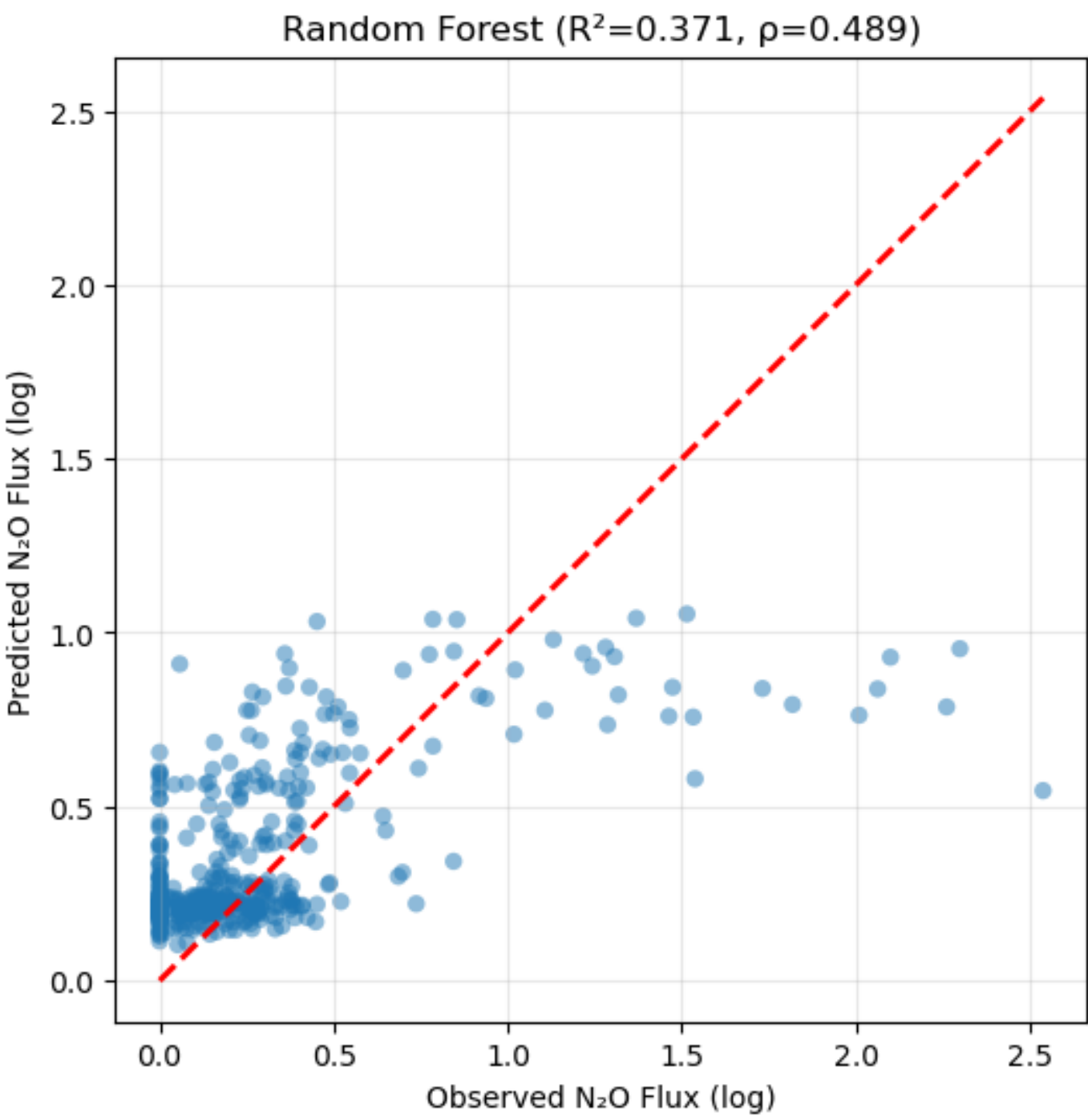
Figure 1: Scatterplot of RF model accuracy for Chamau
