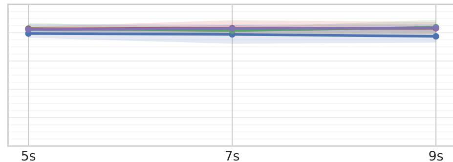
Class 5
