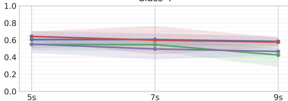
Class 4
