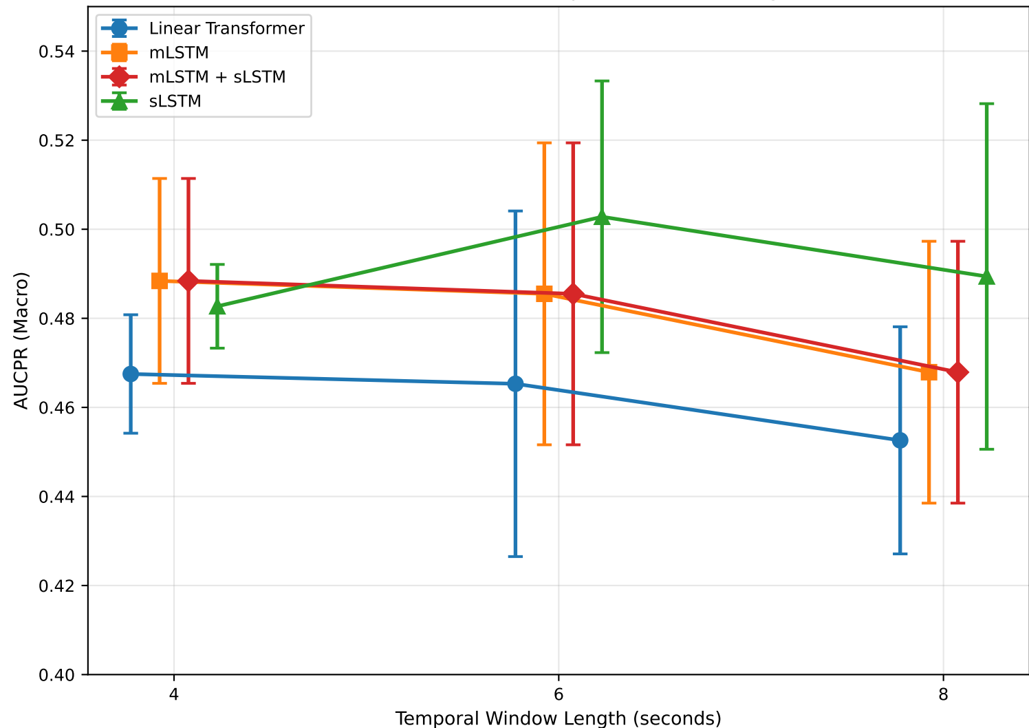
AUCPR (Macro) vs. Temporal Window Length
