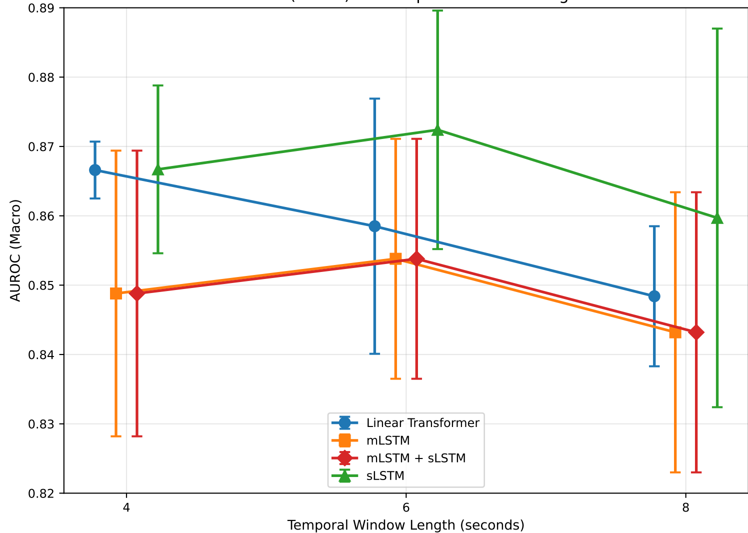
AUROC (Macro) vs. Temporal Window Length
